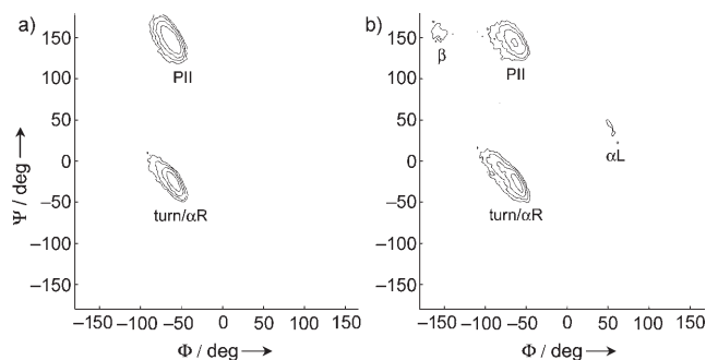
Figure 2. Ramachandran plots of Pro (a) and Ala (b) on the coil library. [18] The mesostates are labeled as PII, \beta , turn/ \alpha R, and \alpha L. The contours are drawn with statistical weights of 0.05%, 0.1%, 0.2%, and 0.4%.
