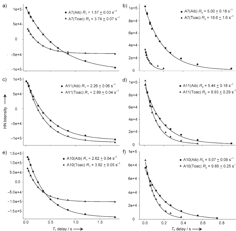
Figure 1. Relaxation data and fitting plots of H^N in ^{15}N -labeled Ala residues. a) R_1 of A*7. b) R_2 of A*7. c) R_1 of A*11. d) R_2 of A*11. e) R_1 of A*10. f) R_2 of A*10.
